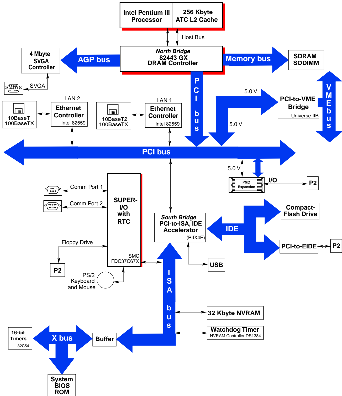
Figure 1. VMIVME-7740 Block Diagram
