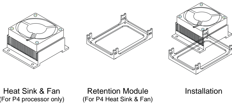
Figure 4: Heat Sink Installation
