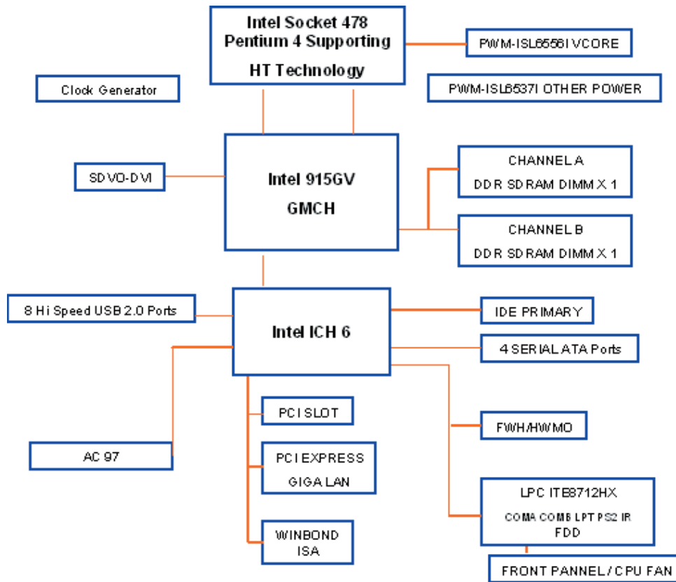
WSB-9150-R10 + Silicon Image Chip + IO-KIT-001 = WSB-9150DVI-R10
