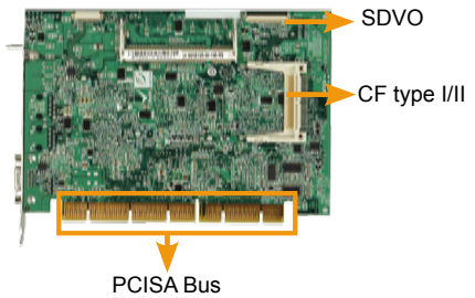
Solder Side
